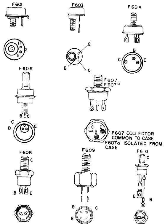
Figure D-1 (7). Transistor outline drawings (part 7 of 20).
