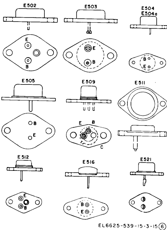
Figure D-1 (6). Transistor outline drawings (Part 6 of 20).
