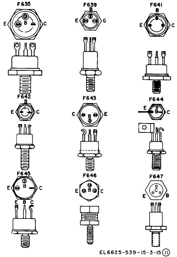
Figure D-1 (11). Transistor outline drawings
