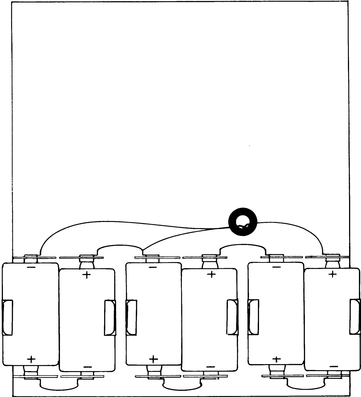
Figure 6-1. Battery polarity and location.
