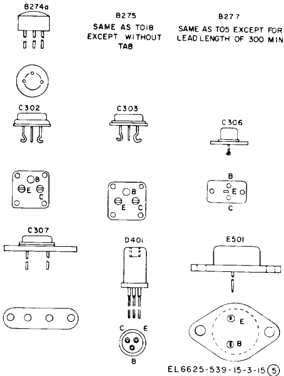
Figure D-1 (5). Transistor outline drawings (part 5 of 20).
