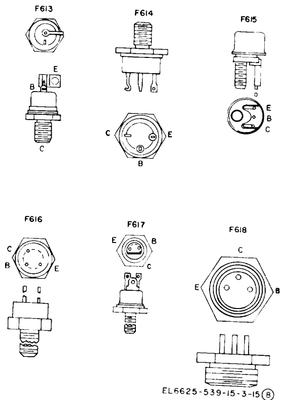
Figure D-1 (8). Transistor outline drawings (part 8 of 20).
