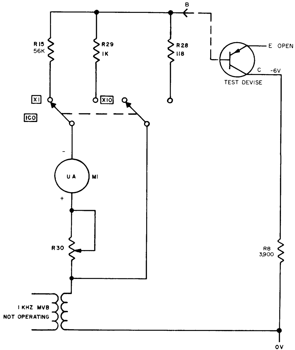
Figure 5-4 I_{co} (leakage) check, simplified schematic diagram.
