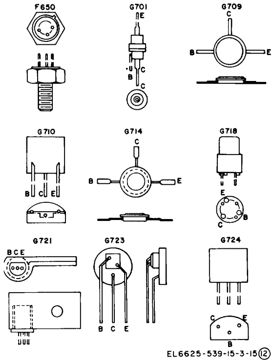
Figure D-1 (12). Transistor outline drawings (part 12 of 20).
